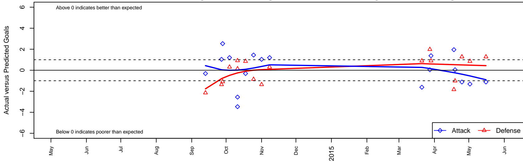
Cheney Storm FC G03 Dots are actual minus expected GF (blue circles) and GA (red triangles). Blue line is smoothed change in attack strength. Red is smoothed change in defense strength.
